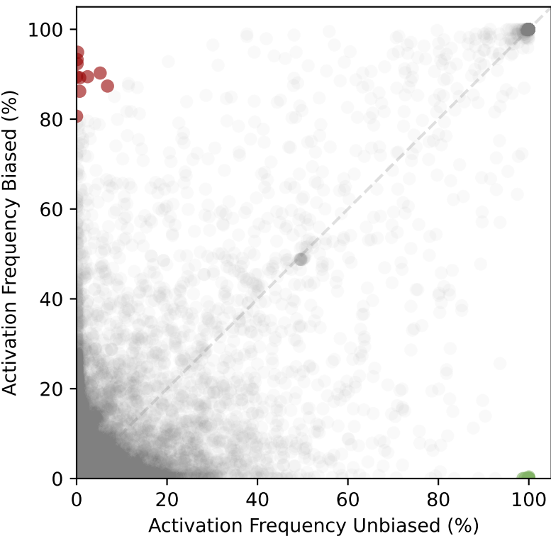
Activation Frequencies of SAE Latents: Gender
